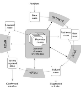
Gambar 1. Proses Case Based Reasoning (CBR)
