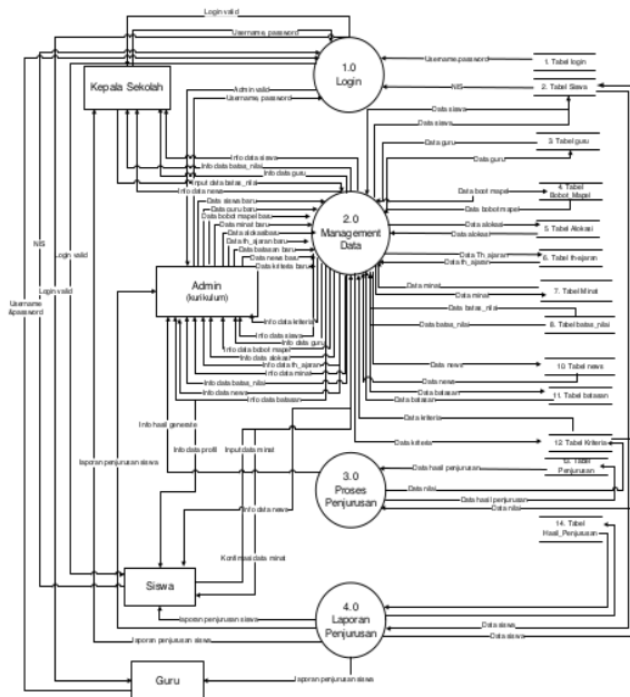
Gambar 3. DFD Level 0
