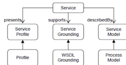
Figure 1. The main concept of OWL-S [9]
