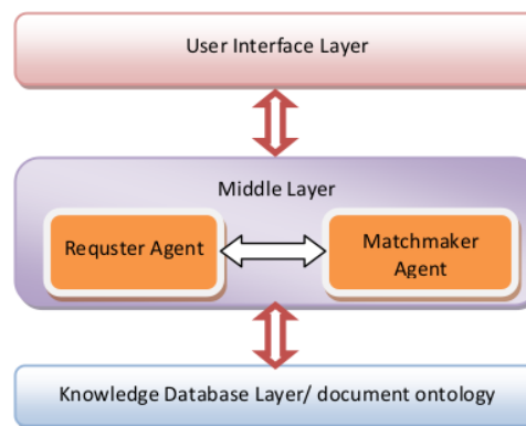
Figure 2. The architecture scheme of the application
