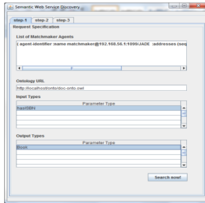
Figure 6. SWS Discovery Display
