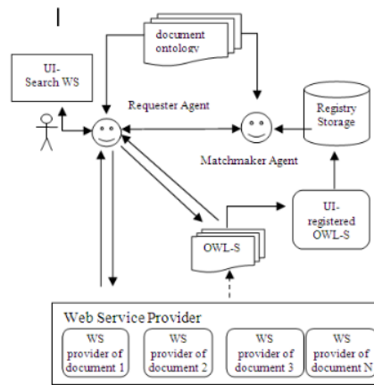
Figure 3. The application flowchart
