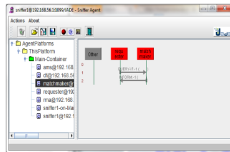
Figure 7. Sniffer Agent.
