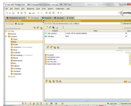
Figure 4. Document Ontology
