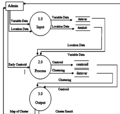
Figure 2. DFD Mapping
