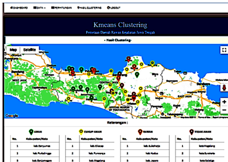
Figure 4. Clustering Results
