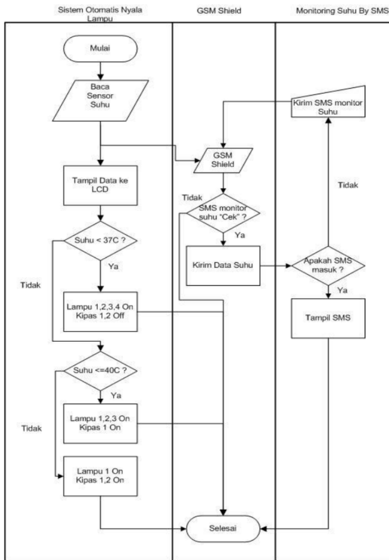
Gambar 6. Flowchart Sistem
