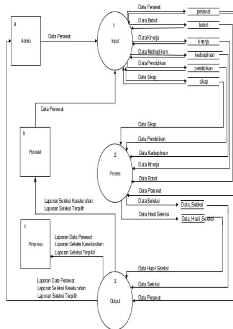
Gambar 3 DAD Level 0
