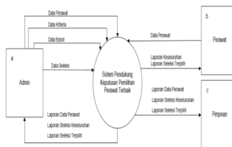
28 Gambar 1 Context Diagram
