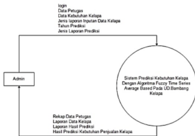
Gambar 1 Diagram Konteks. Data Flow Diagram
