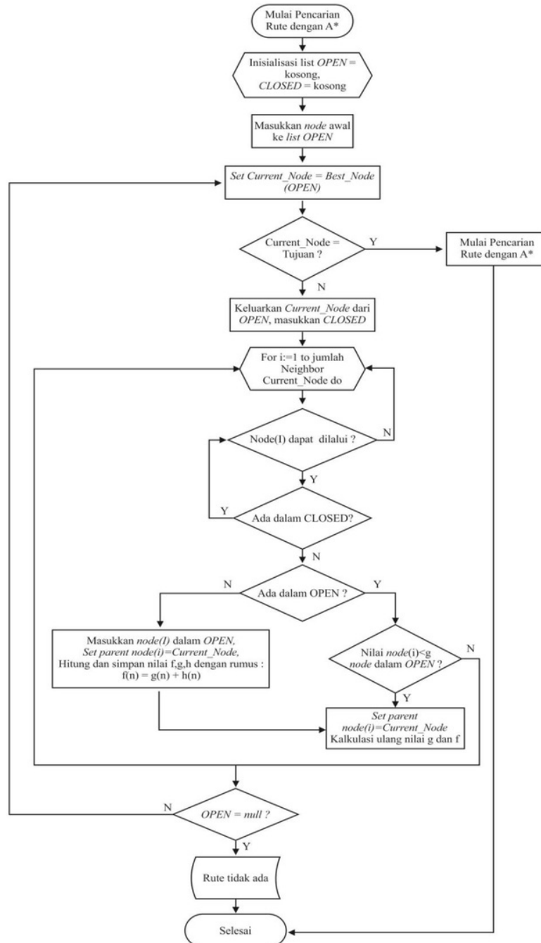
Gambar 2. Flowchart Algoritma A*
