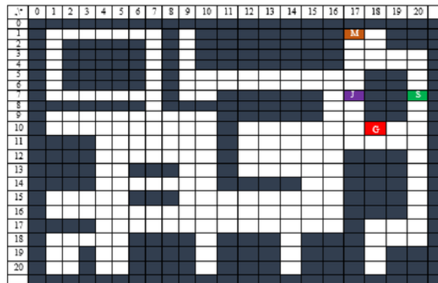
Gambar 3. Arena Game
