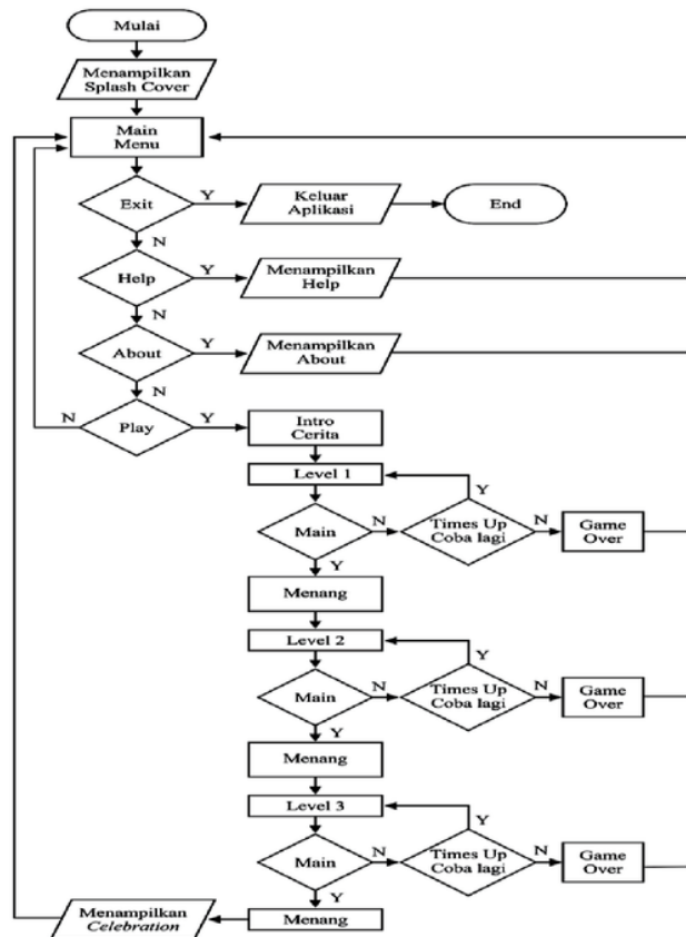
Gambar 1. Flowchart Game
