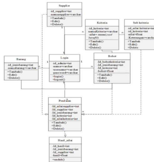
Gambar 2. Class Diagram
